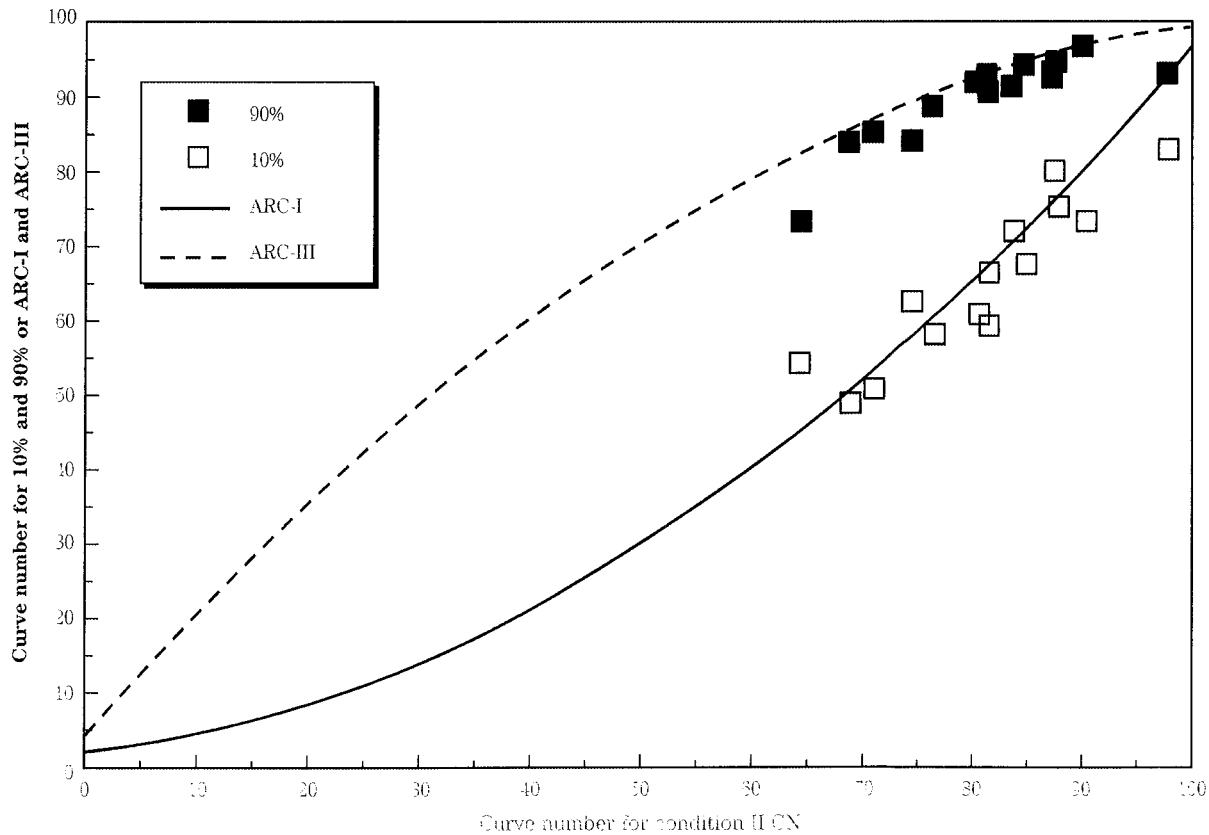
Figure 10-4 Comparison of 10 and 90 percent extremes with ARC I and ARC III values from table 10-1 (adapted from Hjelmfelt 1991)
